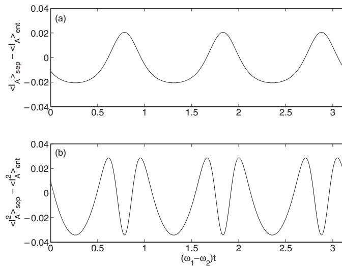
Figure 4. (a) \langle \hat{I}_A \rangle_{\text{sep}} - \langle \hat{I}_A \rangle_{\text{ent}} and (b) \langle \hat{I}_A^2 \rangle_{\text{sep}} - \langle \hat{I}_A^2 \rangle_{\text{ent}} against (\omega_1 - \omega_2)t for the coherent state \rho_{\text{sep},A} of equation (42) and \rho_{\text{ent},A} of equation (45) with A_1 = \sqrt{2} , A_2 = 0 . The photon frequencies are \omega_1 = 1.2 \times 10^{-4} and \omega_2 = 10^{-4} , in units where k_B = \hbar = c = 1 .
