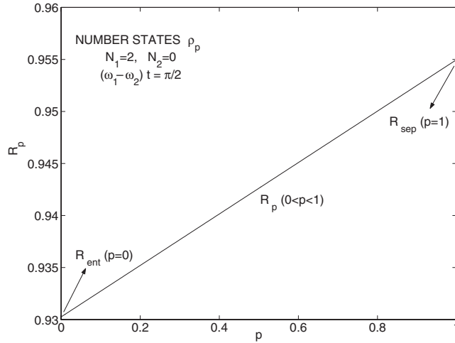
Figure 6. R_p against p for currents that are induced by the interpolating density matrix \rho_p of equation (22) for number states with N_1 = 2, N_2 = 0 . The time t has been fixed so that (\omega_1 - \omega_2)t = \pi/2 . The photon frequencies are \omega_1 = 1.2 \times 10^{-4} and \omega_2 = 10^{-4} , in units where k_B = \hbar = c = 1 .
