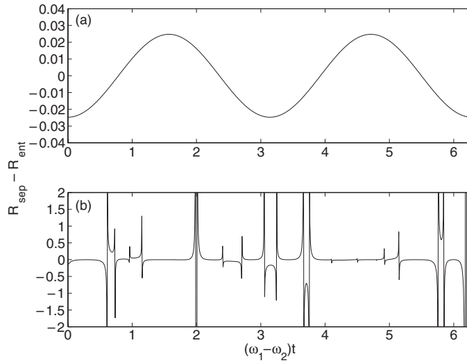
Figure 3. R_{\text{sep}} - R_{\text{ent}} against (\omega_1 - \omega_2)t for (a) number states of equations (20) and (21) with N_1 = 2 , N_2 = 0 and (b) coherent states of equations (39) and (40) with A_1 = \sqrt{2} , A_2 = 0 . The photon frequencies are \omega_1 = 1.2 \times 10^{-4} and \omega_2 = 10^{-4} , in units where k_B = \hbar = c = 1 .
