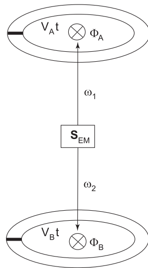
Figure 1. Two distant mesoscopic SQUID rings A and B are irradiated with nonclassical microwaves of frequencies \omega_1 and \omega_2 , respectively. The microwaves are produced by the source S_{EM} and are correlated. Classical magnetic fluxes V_A t and V_B t are also threading the two rings A and B, respectively.
