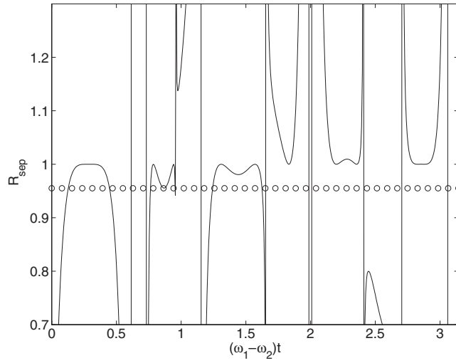
Figure 2. R_{\text{sep}} against (\omega_1 - \omega_2)t for the number state of equation (20) with N_1 = 2 , N_2 = 0 (line of circles) and the coherent state of equation (39) with A_1 = \sqrt{2} , A_2 = 0 (solid line). The photon frequencies are \omega_1 = 1.2 \times 10^{-4} and \omega_2 = 10^{-4} , in units where k_B = \hbar = c = 1 .
