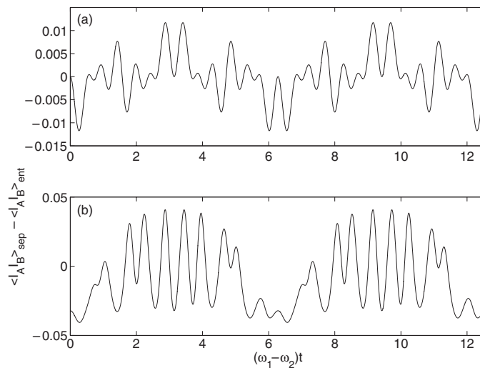
Figure 5. \langle \hat{I}_A \hat{I}_B \rangle_{\text{sep}} - \langle \hat{I}_A \hat{I}_B \rangle_{\text{ent}} for (a) number states of equations (20) and (21) with N_1 = 2 , N_2 = 0 and (b) coherent states of equations (39) and (40) with A_1 = \sqrt{2} , A_2 = 0 , against (\omega_1 - \omega_2)t . The photon frequencies are \omega_1 = 1.2 \times 10^{-4} and \omega_2 = 10^{-4} , in units where k_B = \hbar = c = 1 .
